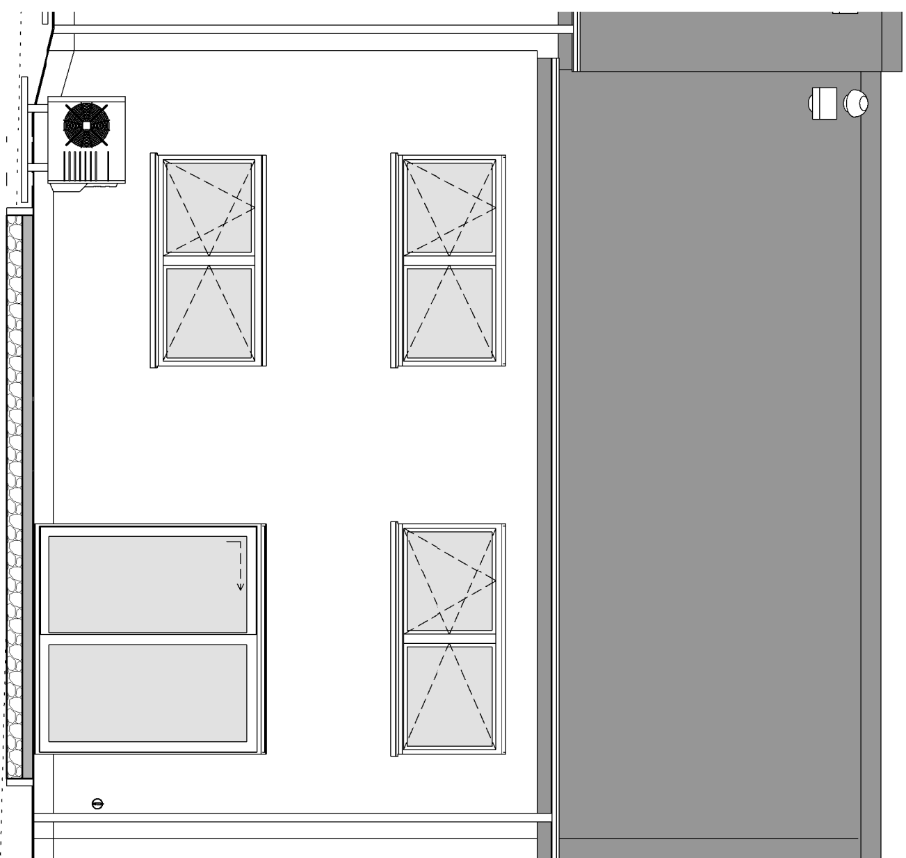
FACADE ARRIERE
